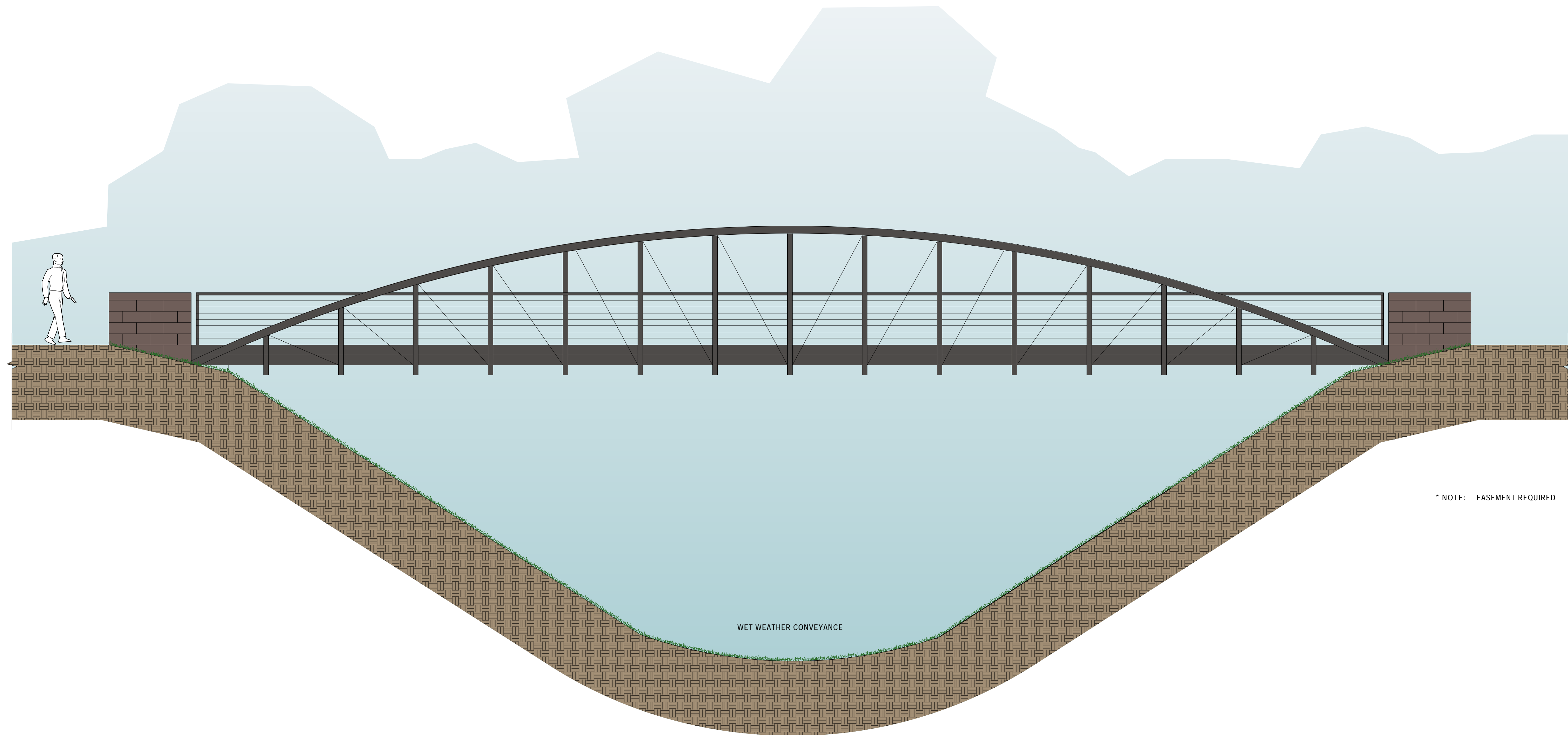
5 BRIDGE AT DRAINAGE SWALE (50' LENGTH) SCALE: 1/4"=1'-0" @ / NEAR INGERSOLL AVE. @ / NEAR LESTER RD.
