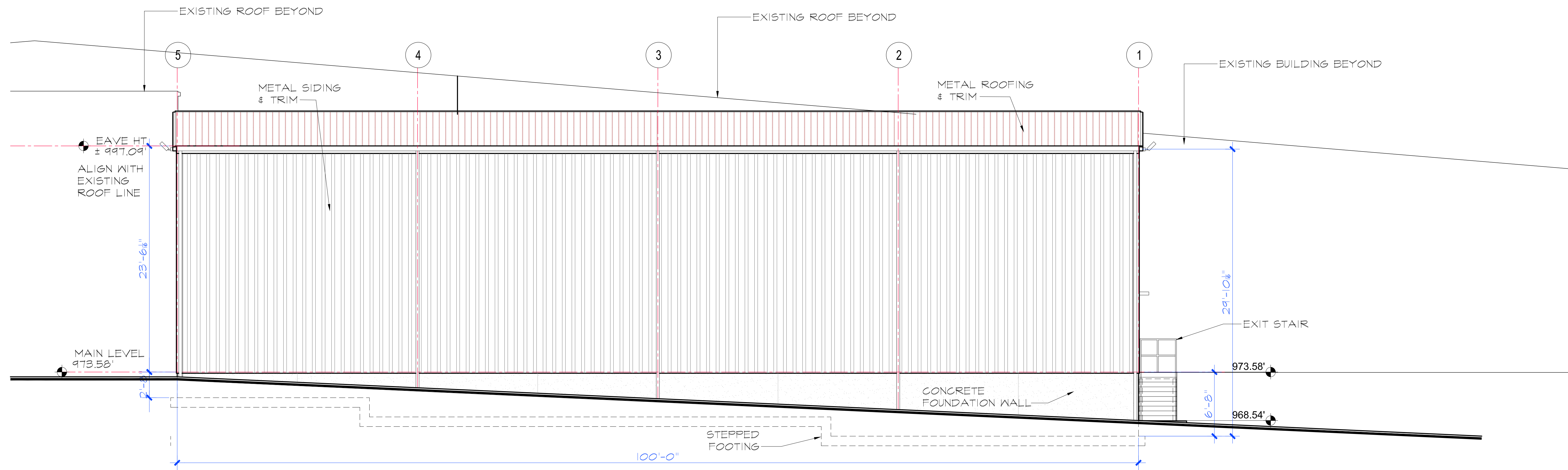
1 NORTHWEST ELEVATION - WAREHOUSE ADDITION A2 22SEP21
